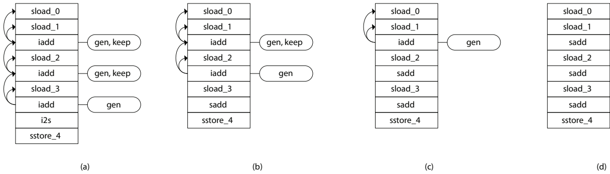
Figure 7. Arithmetic optimisation.
