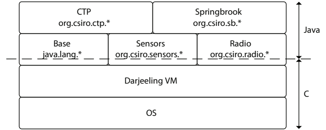
Figure 12. Software stack.
