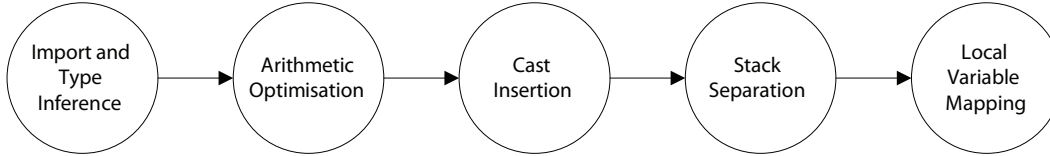
Figure 5. byte code transformation pipeline.
