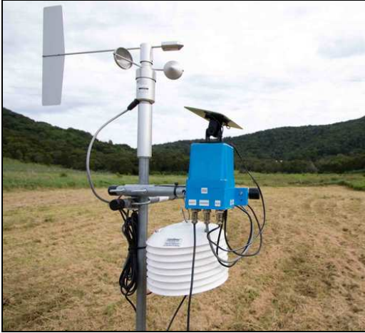
Figure 11. The environmental monitoring node which measures soil moisture, leaf wetness, wind speed and direction, temperature and humidity.
